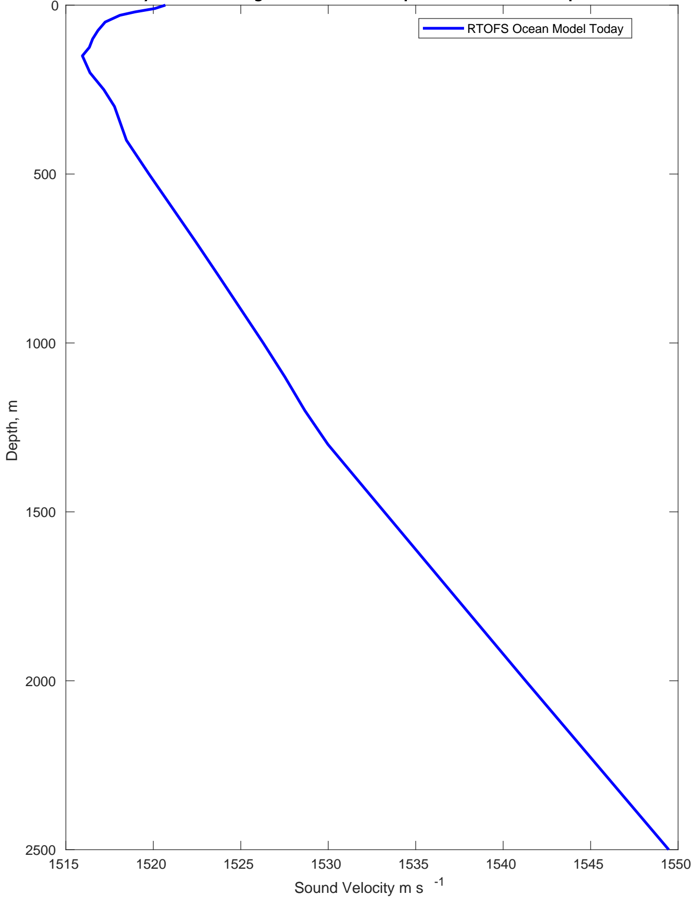
Sound Velocity Profile for Lighthouse Greece Pipeline-OSS2 on 24-Apr-2022 00:00:00
